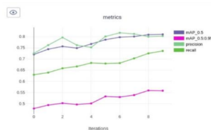
Fig 6- Model Performance Metric
