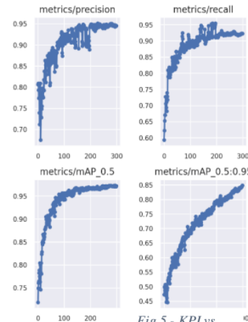
Fig 5 - KPI vs Iterations
